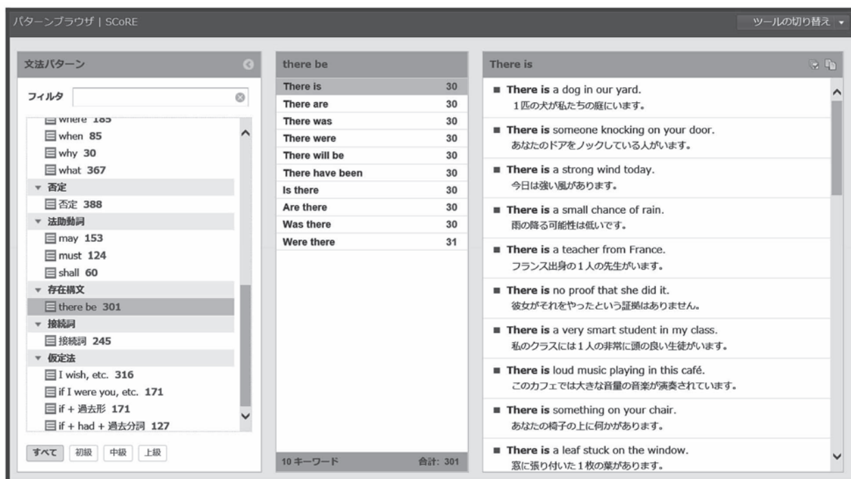
Fig. 1 Screenshot of the Pattern Browser Showing a Search for “There is”
