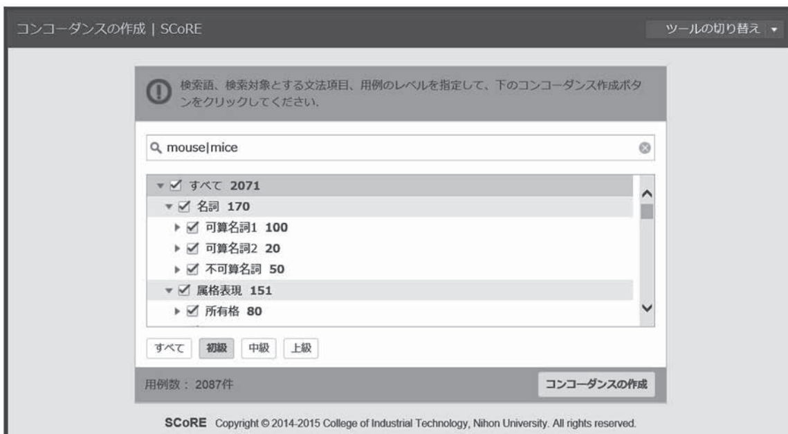
Fig. 4 Screenshot of the Concordance Setting Searching for Beginner Level “mouse|mice”
